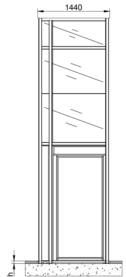
Section G-G
