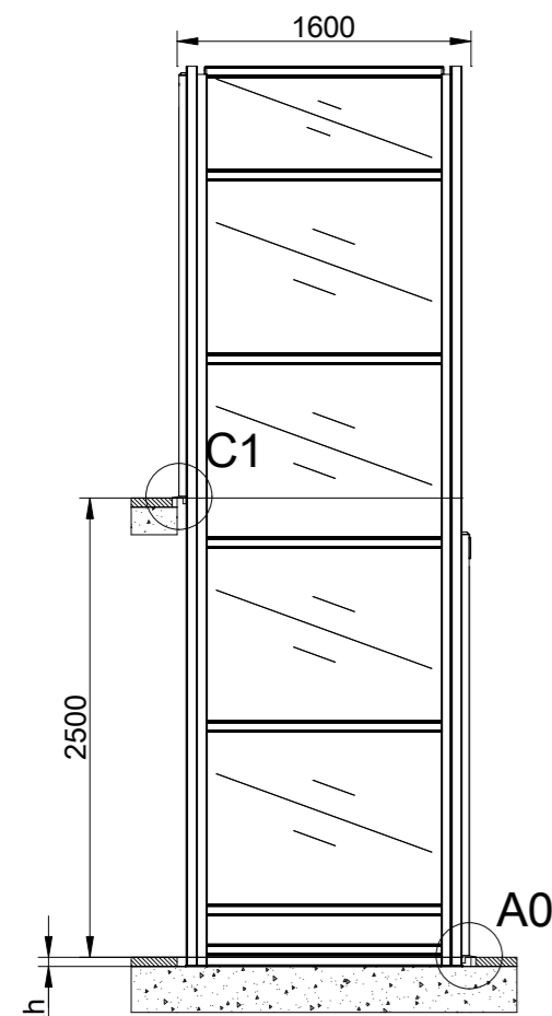
Section E-E
